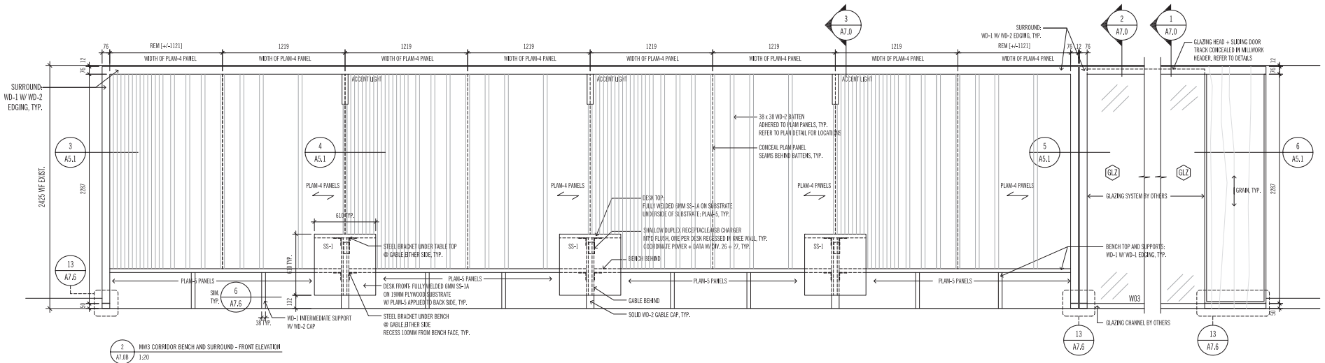
CONSTRUCTION DRAWINGS- CORRIDOR BENCH/SURROUND MILLWORK PLAN & ELEVATION (AUTOCAD)
