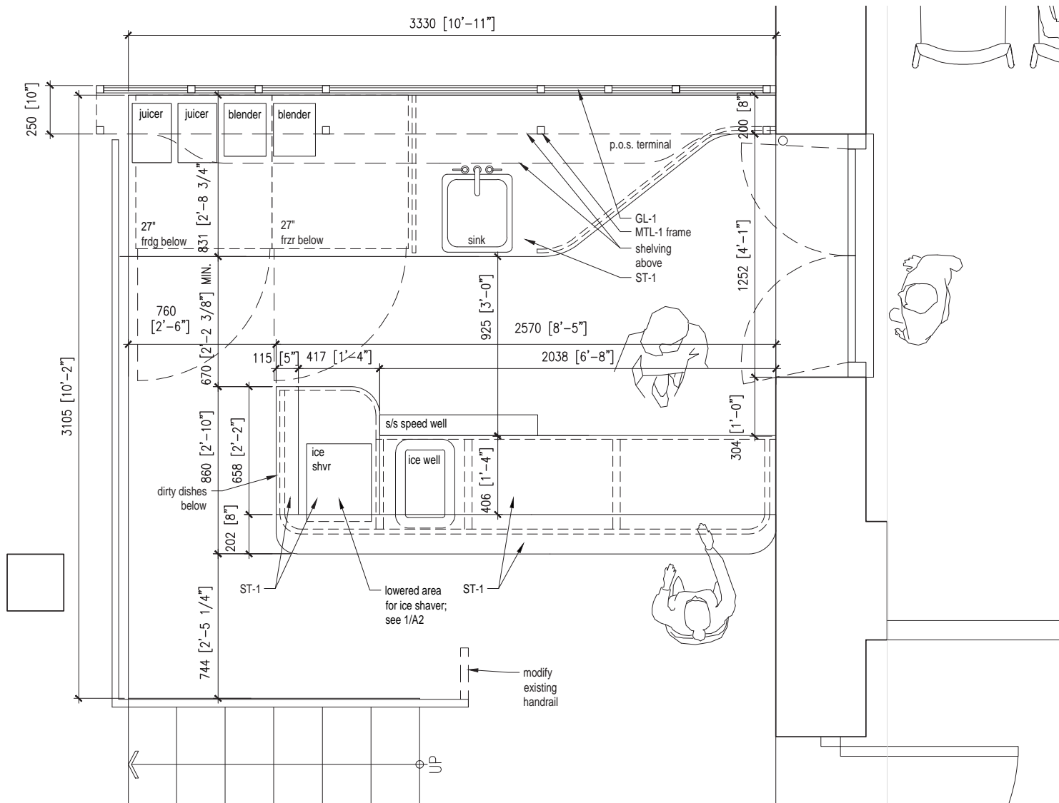
CONSTRUCTION DRAWINGS - WET BAR PLAN (AUTOCAD)
