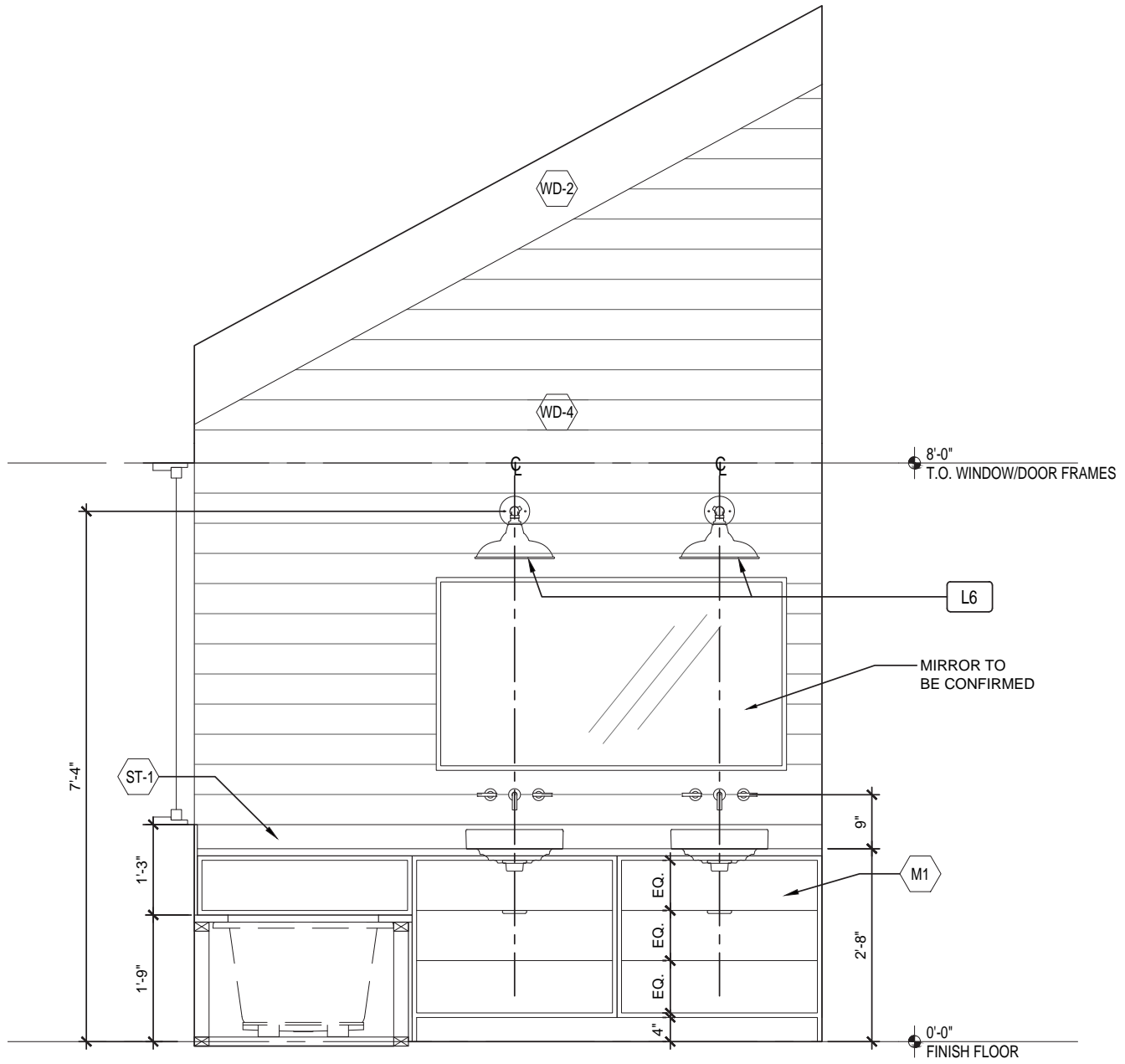
CONSTRUCTION DRAWINGS- PRIMARY BATH INTERIOR ELEVATION (AUTOCAD)
