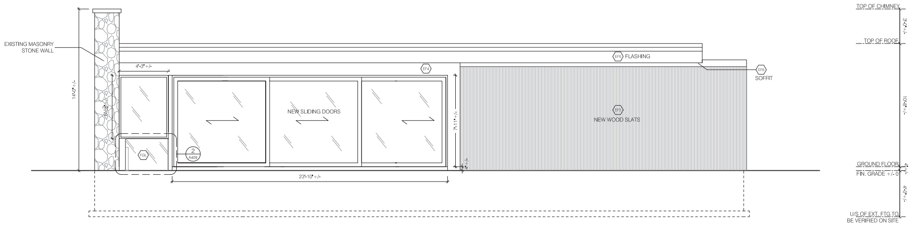
1 Front Elevation SCALE: 3/16" = 1'-0"
