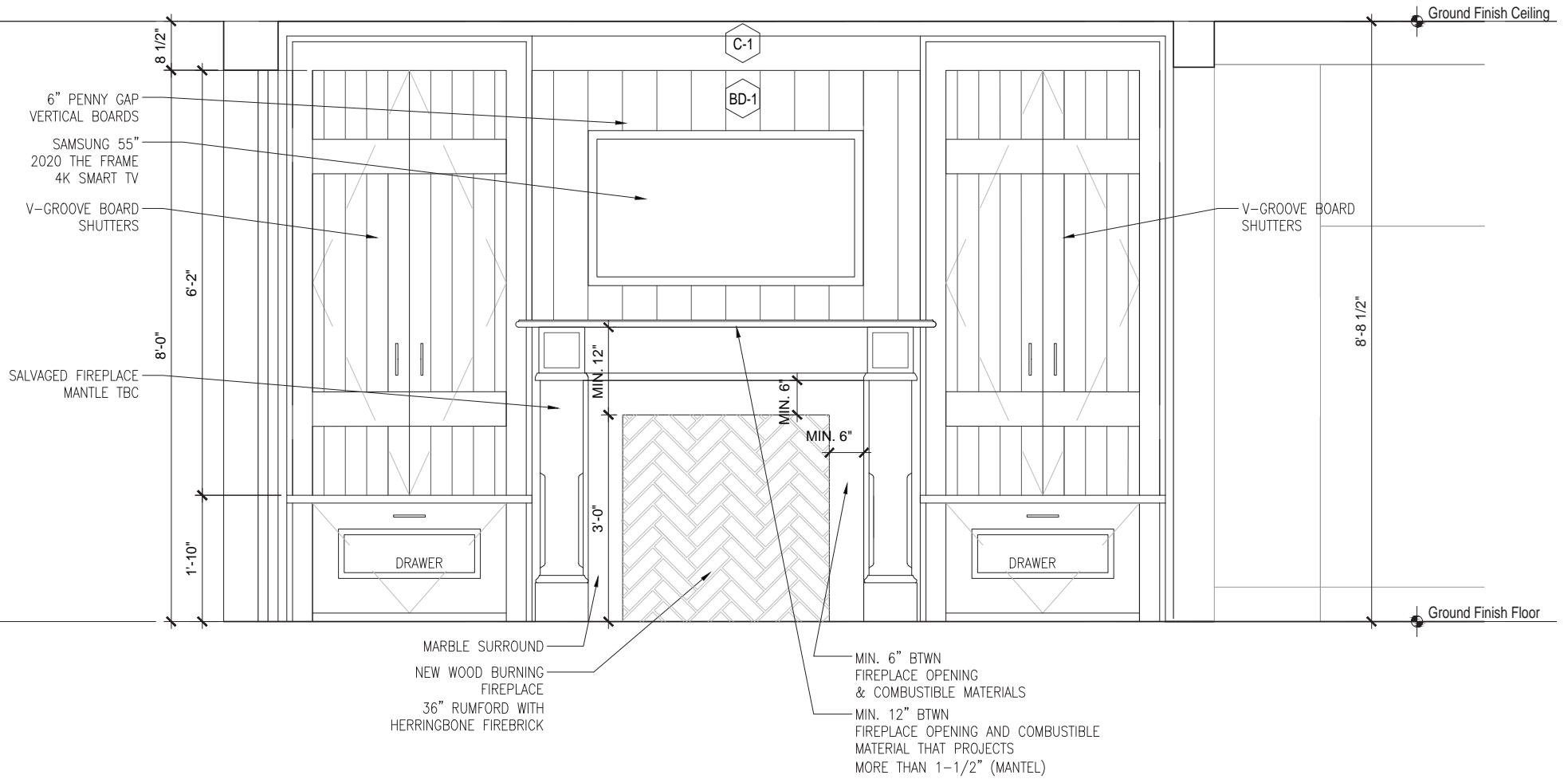
CONSTRUCTION DRAWINGS- LIVING ROOM INTERIOR ELEVATION (AUTOCAD)
