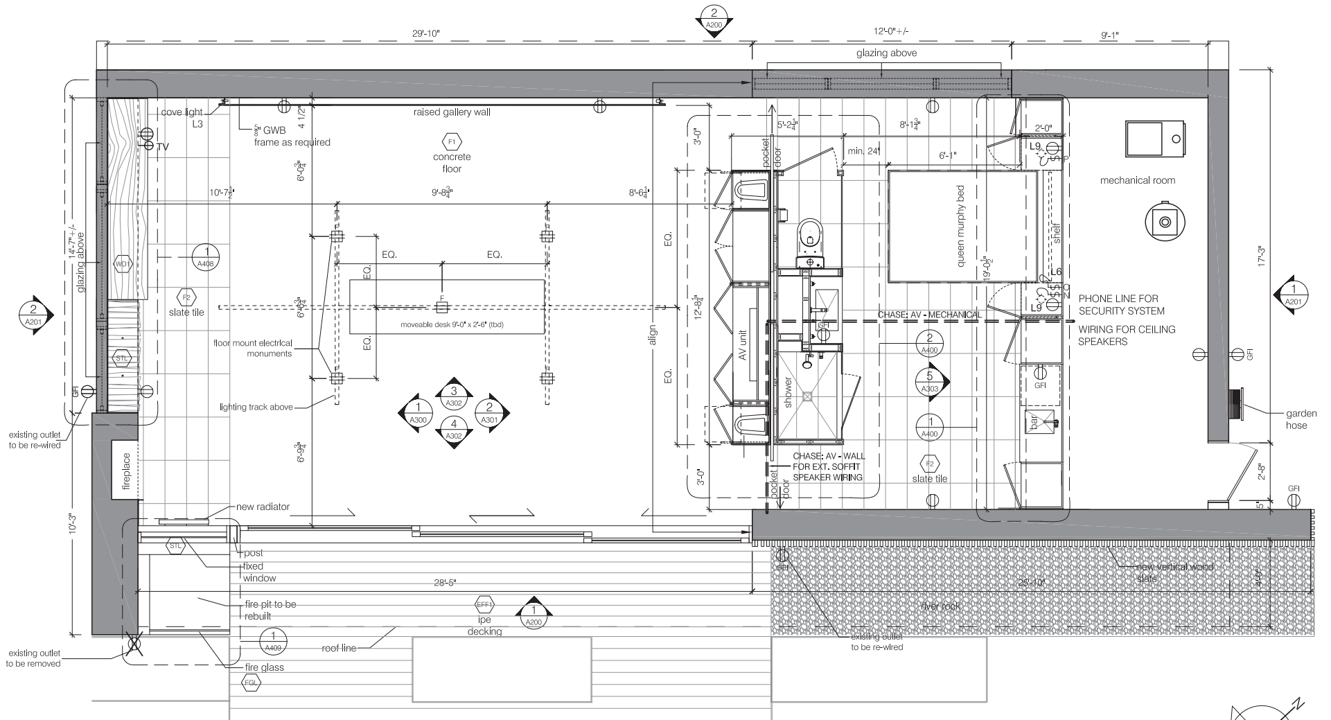
CONSTRUCTION DRAWINGS - PLAN (AUTOCAD)
