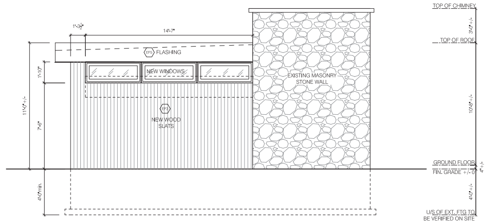
2 Side Elevation SCALE: 3/16" = 1'-0"
