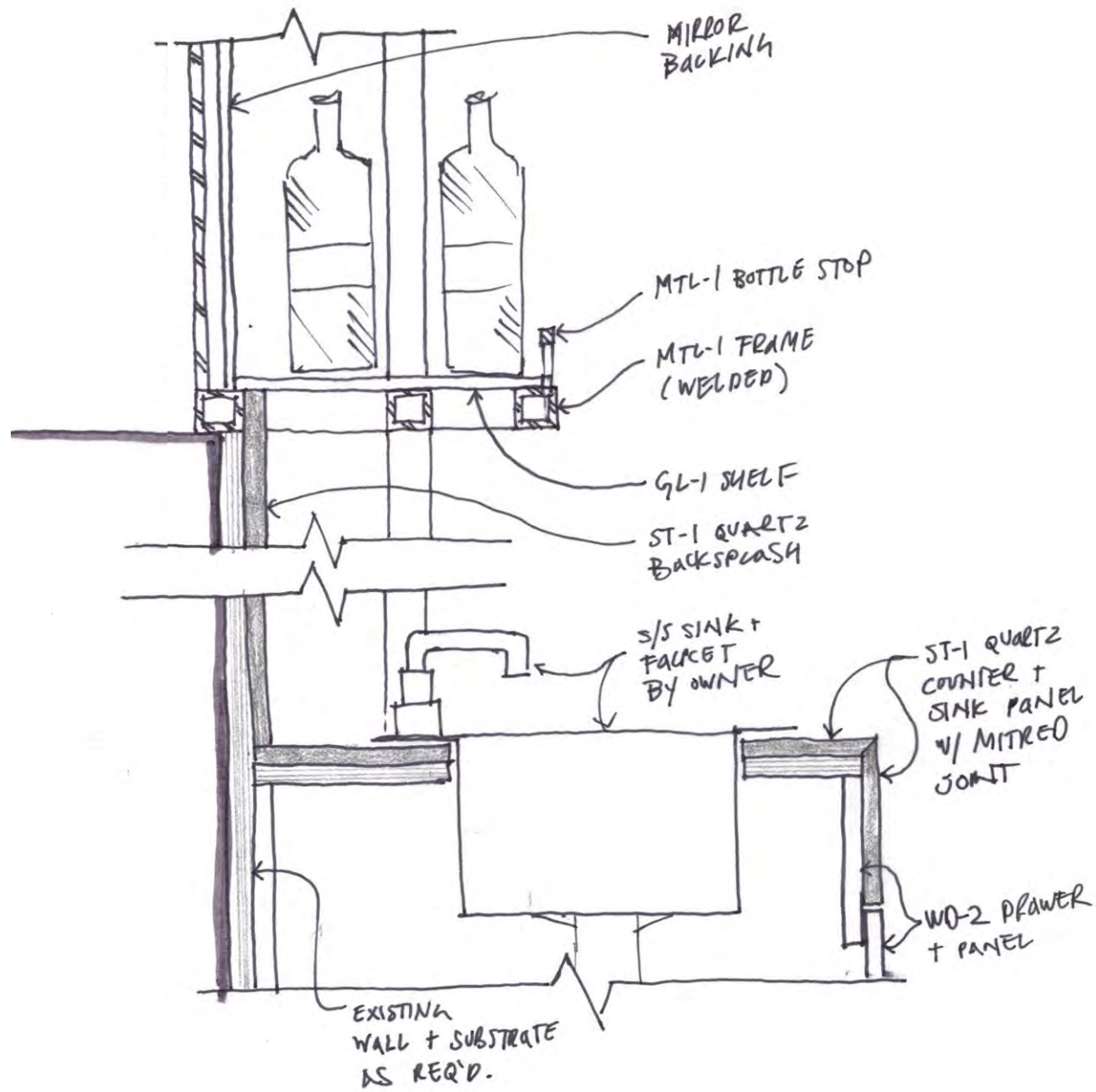
MILLWORK DETAIL SKETCH (BY HAND)
