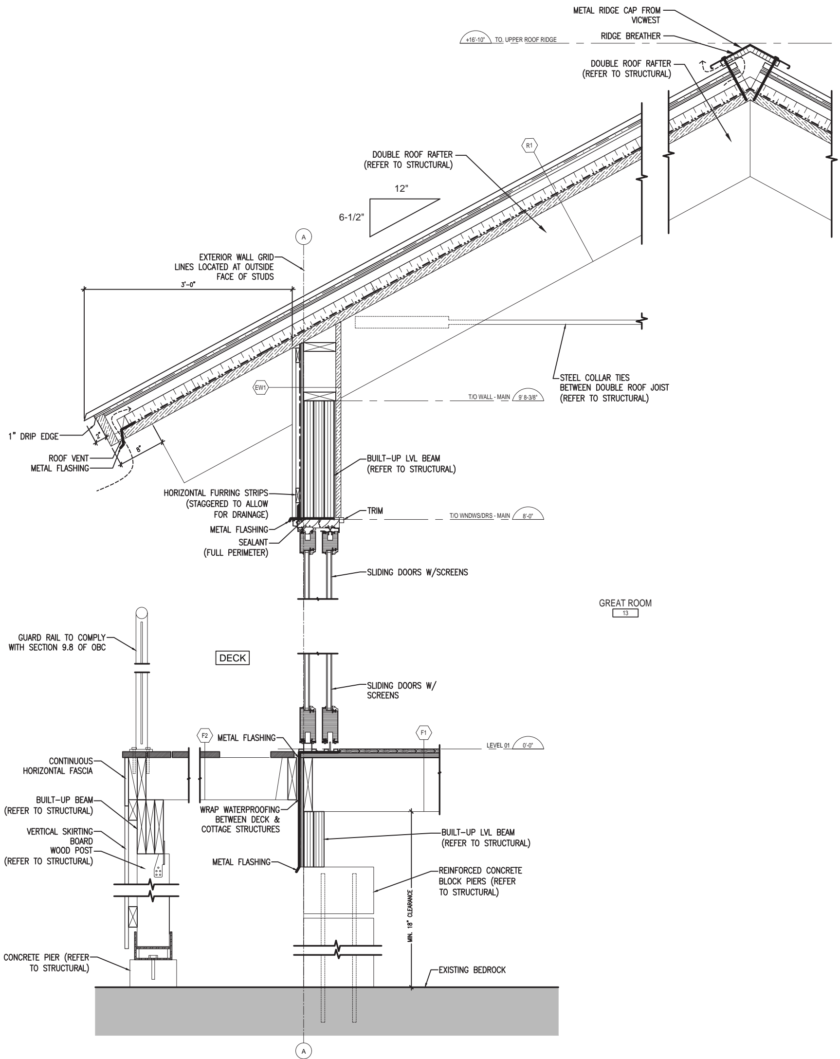
Typical Wall Section - Great Room
