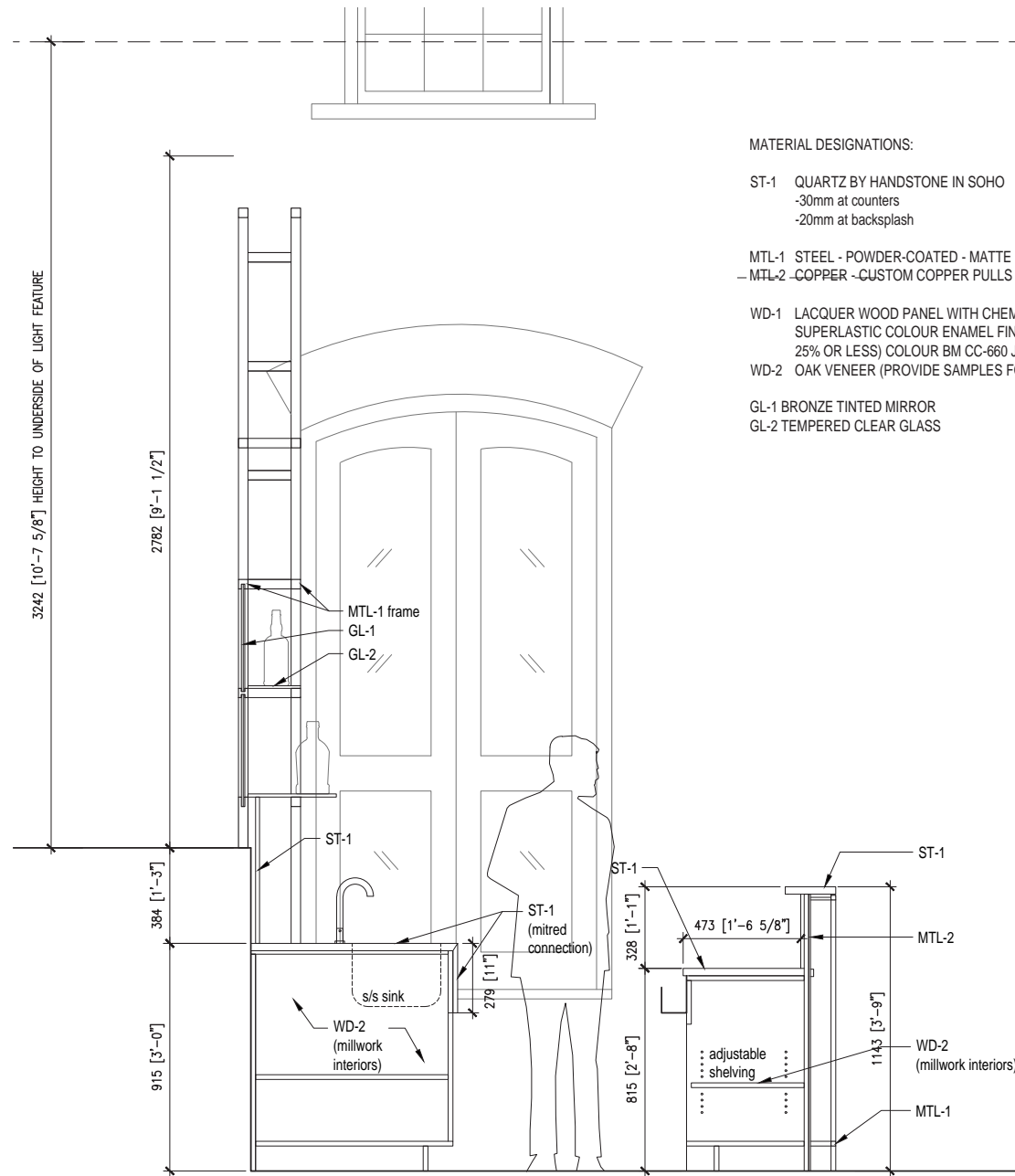
CONSTRUCTION DRAWINGS - WET BAR SECTION (AUTOCAD)
