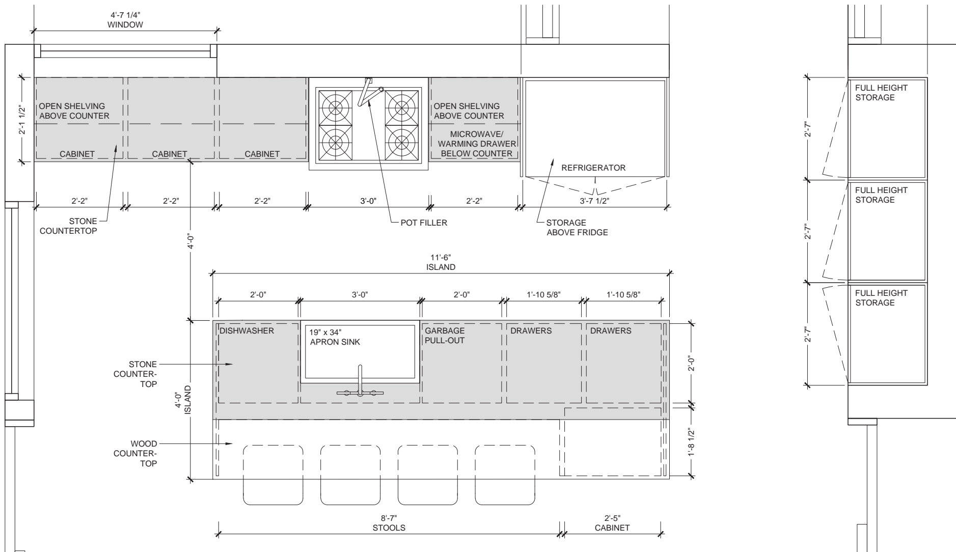
KITCHEN PLAN (AUTOCAD)
