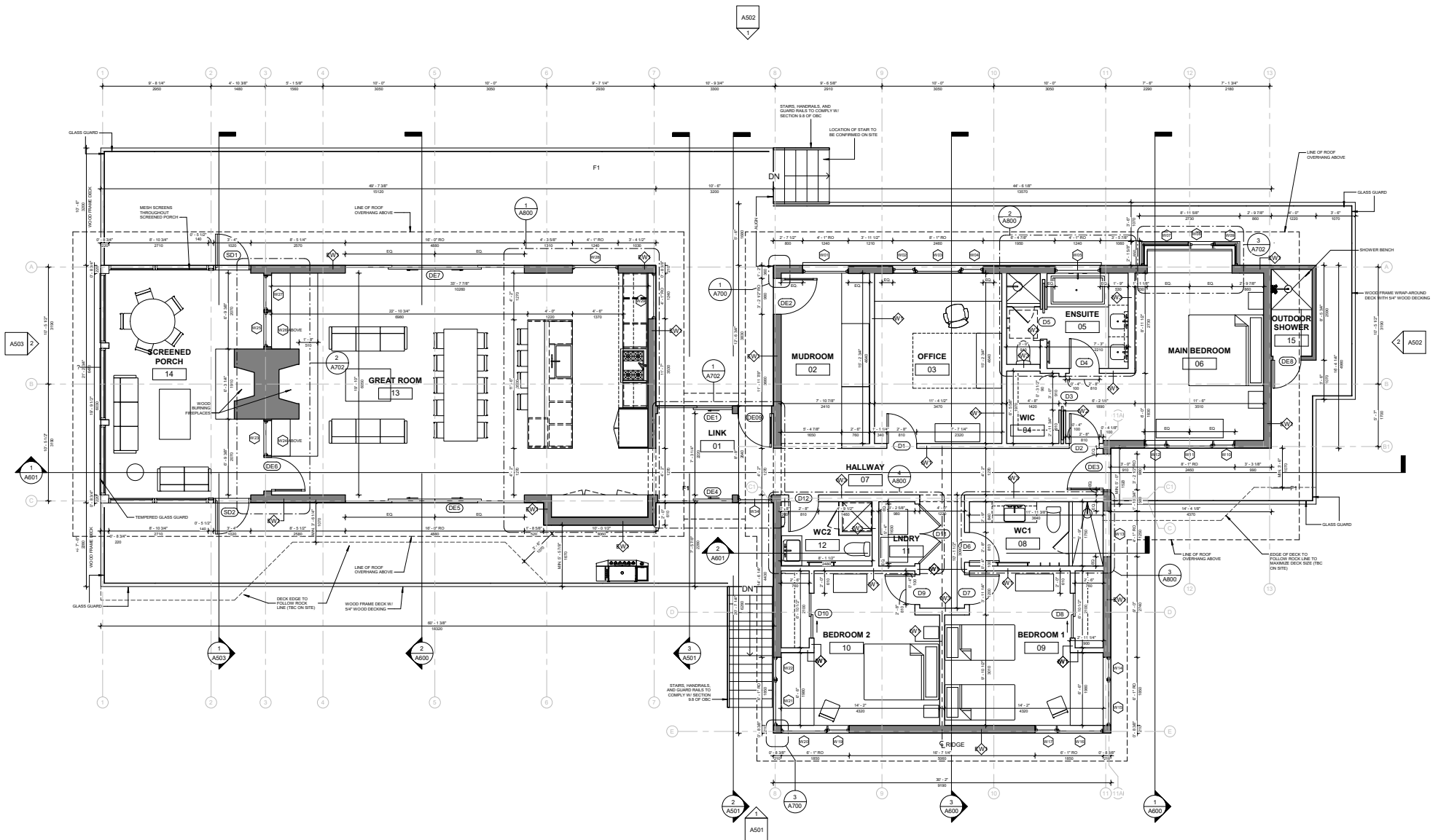
CONSTRUCTION DRAWINGS - COTTAGE PLAN (REVIT)
