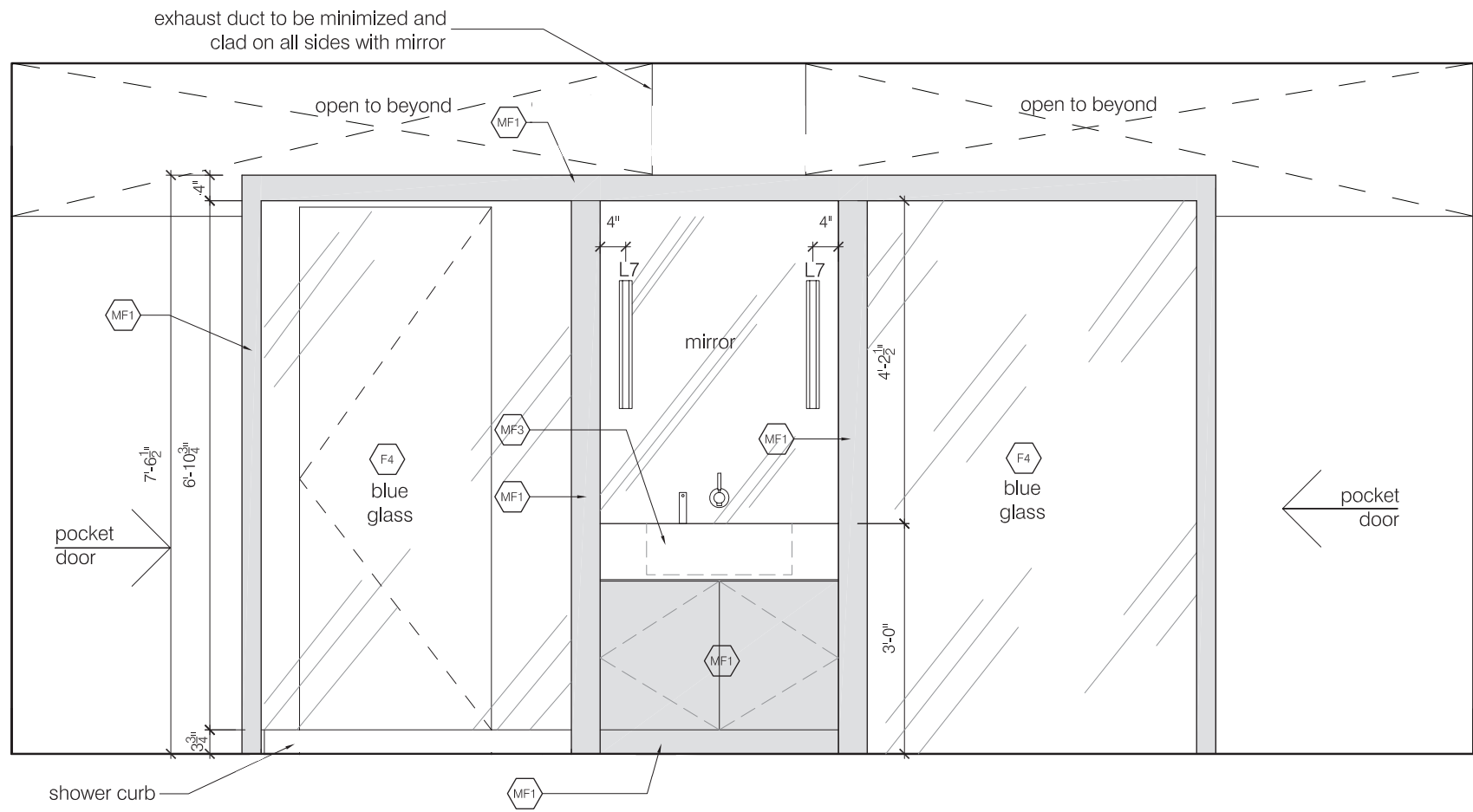
CONSTRUCTION DRAWINGS - CENTRE MILLWORK WASHROOM-SIDE ELEVATION (AUTOCAD)
