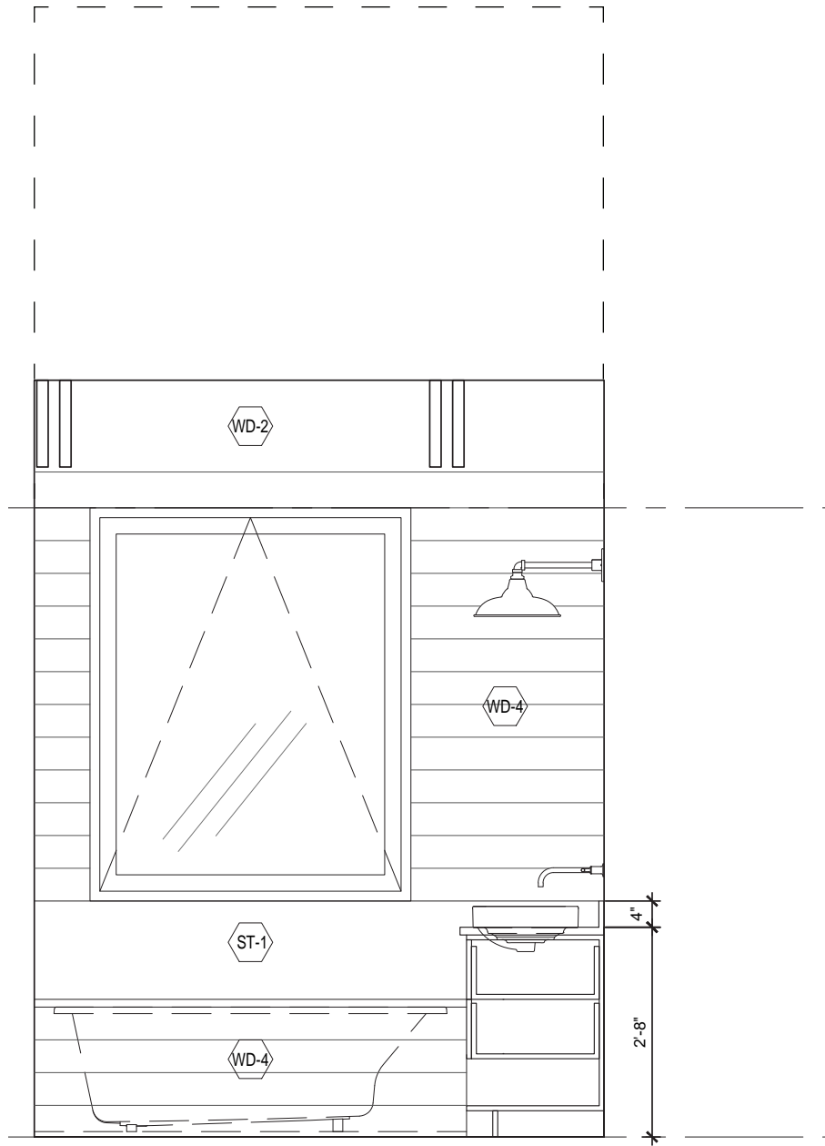
CONSTRUCTION DRAWINGS- PRIMARY BATH INTERIOR ELEVATION (AUTOCAD)
